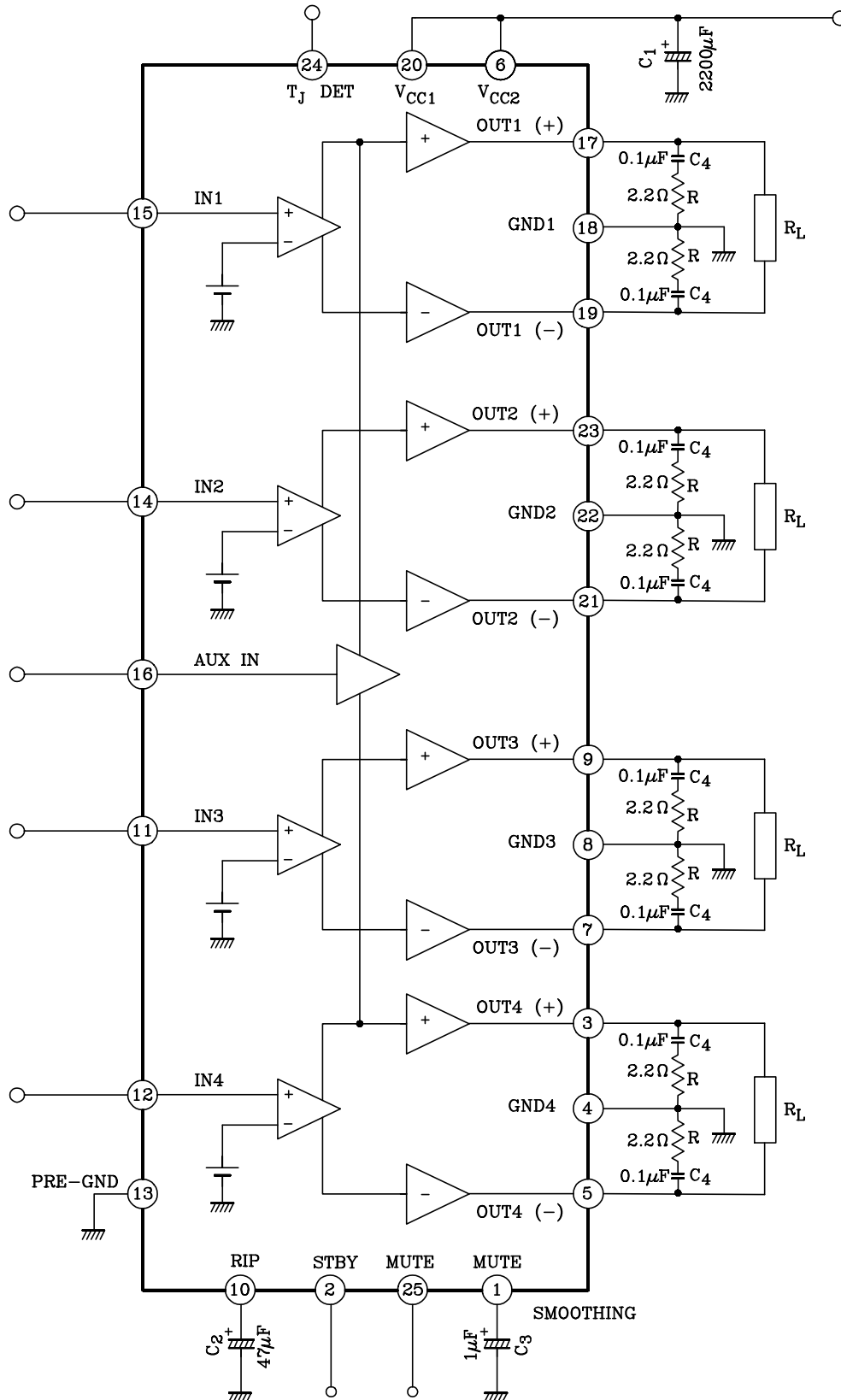
TEST CIRCUIT ( G_V=34\text{dB} )
