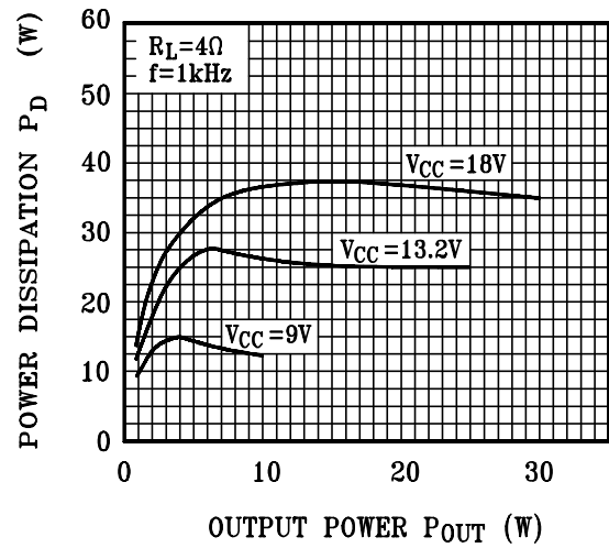
P_D - R_{OUT}
